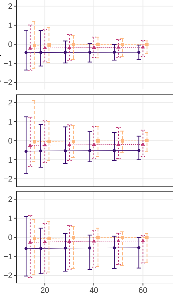
Difference in ICCs to Benchmark (ICC.z)
